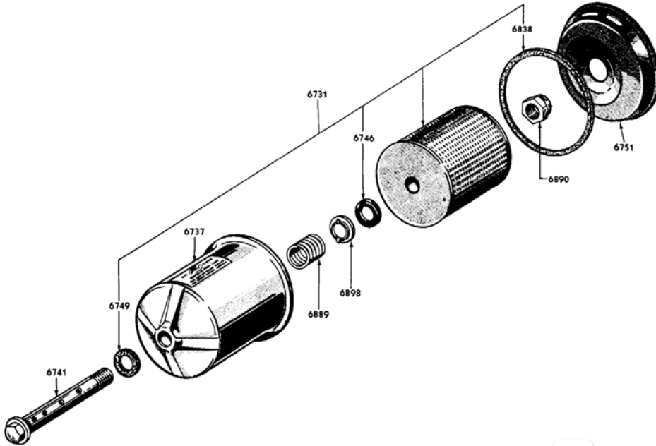
1952/ OIL FILTER & RELATED PARTS (6 CYLINDER 215, 223), (8 CYLINDER 239, 272, 312 "O. H. V." ENGINES)-TYPICAL
