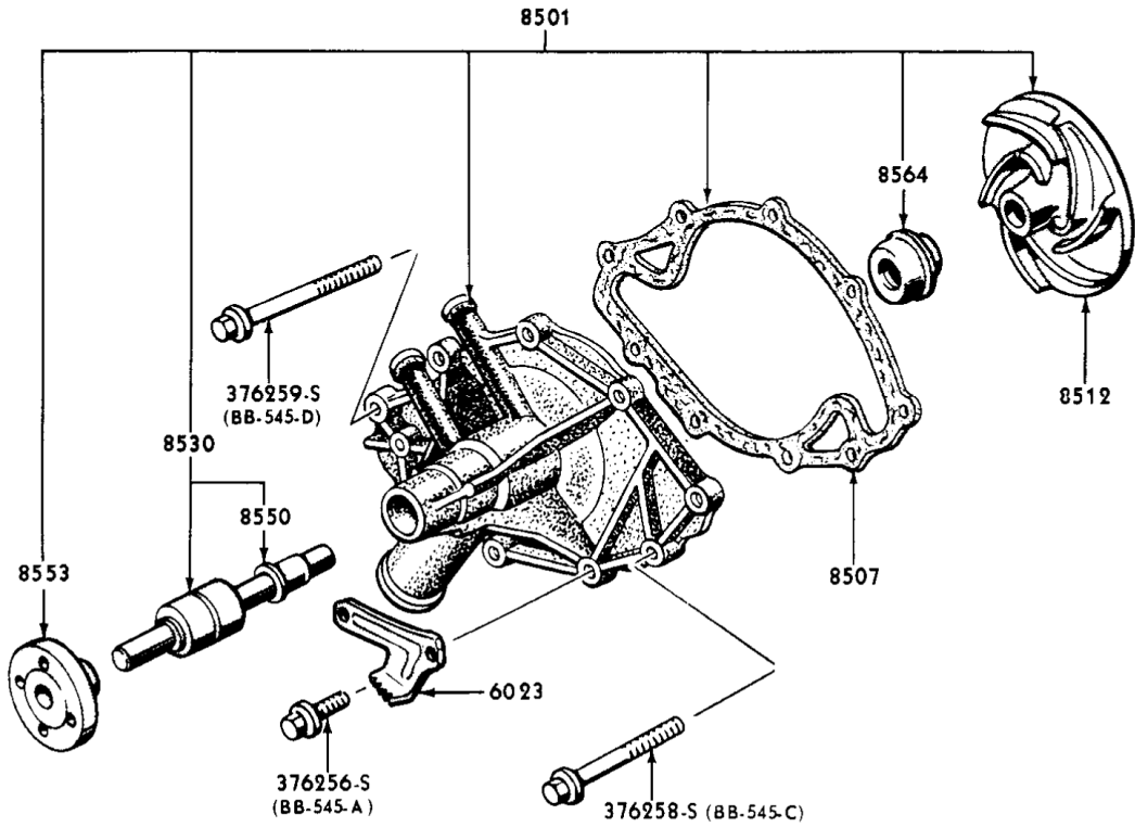
1962 Water Pump (221, 260, 289 V-8)
