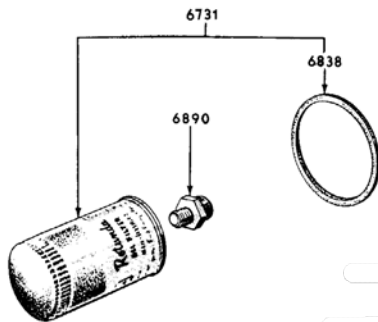
1952/ OIL FILTER & RELATED PARTS (6 CYLINDER 215, 223), (8 CYLINDER 239, 272, 292, 312 "O. H. V." ENGINES)-DISPOSABLE TYPE
